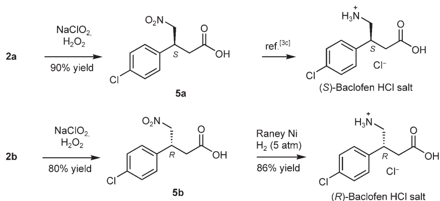
Scheme 2. Synthesis of ( S )- and ( R )-baclofens ( 1 ).
