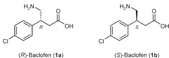
Figure 1. The structures of chiral baclofen ( 1 ).
